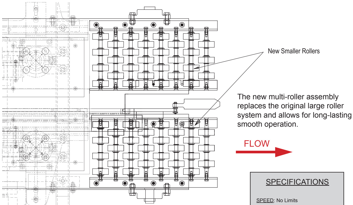
Figure 1.3 - Top View of the new Multi-Roller Assembly
