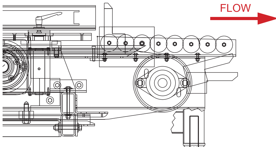
Figure 1.4 - Side View of the new Multi-Roller Assembly
