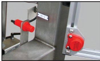
RFID safety interlocked guard door switches stop machine when opened
