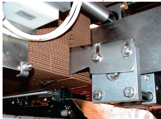
Figure 1.2 - Tray Blank Indexer properly adjusted
