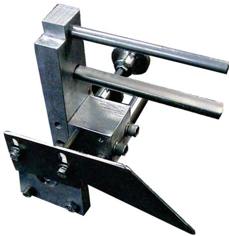
Figure 1.1 - Tray Blank Indexer (Two(2) required)
