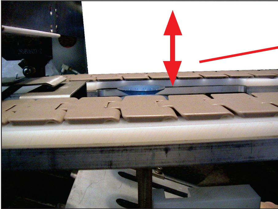
Figure 1.3 - Vacuum Cups shown in down position
