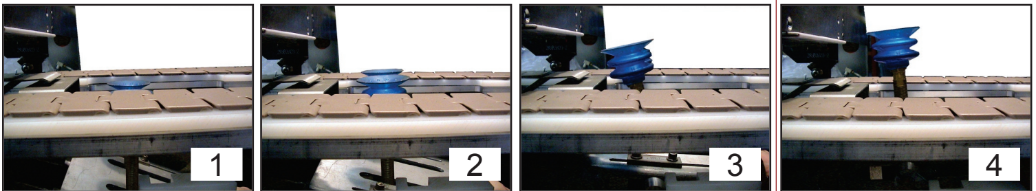
Figure 1.2 - Cam Driven Vacuum Cups (Shown at four stages of motion)
