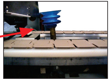
Figure 1.4 - Increased Stroke of vacuum cups traveling upward.
