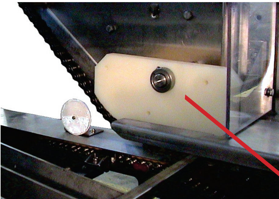
Figure 1.1 - Hi-Fax Plastic Chain Guide
