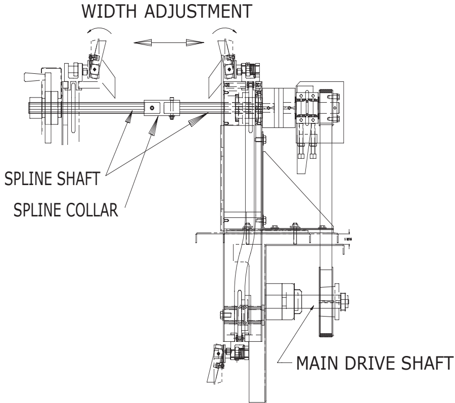
Figure 1.3 - Split Spline Shaft shown with Spline Collar
