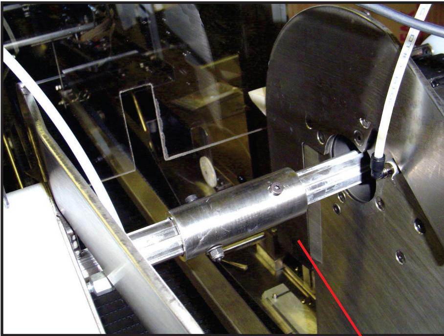
Figure 1.1 - Split Spline Shaft installed on Slitter/Sealer
