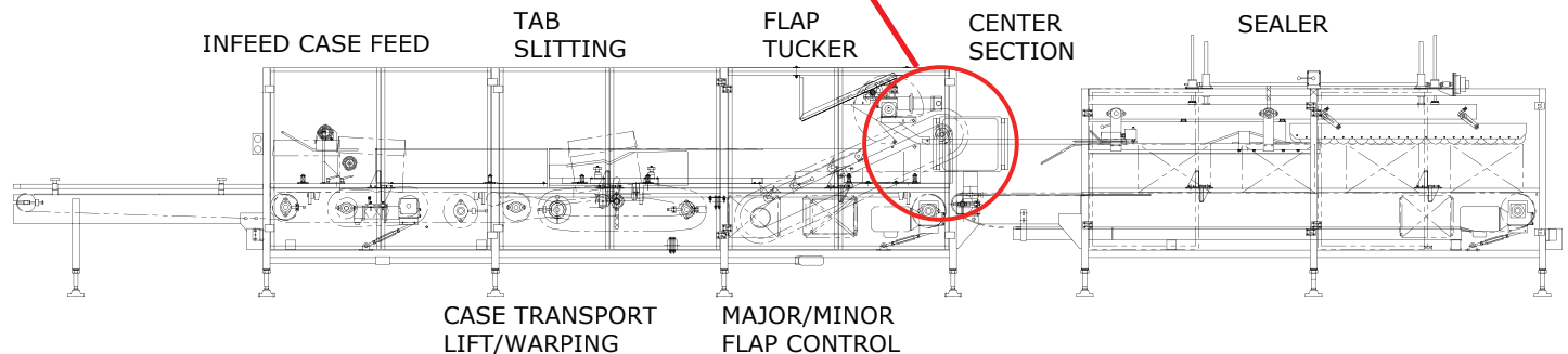
Figure 1.2 - Location of Split Spline Shaft on Slitter/Sealer
