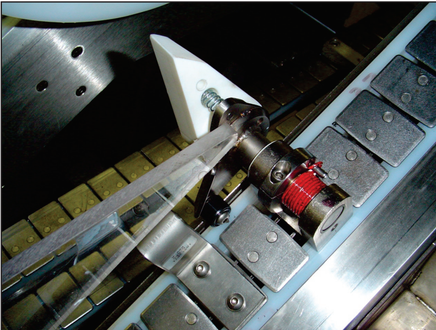
Figure 1.1 - Articulating Tear-Drop installed on Slitter-Sealer
